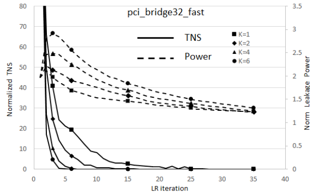
Figure 3.2: TNS and power profiles for different values of K for critical arcs during the timing recovery stage are shown. TNS has been normalized with respect to T . As K increases, TNS reduces faster.
